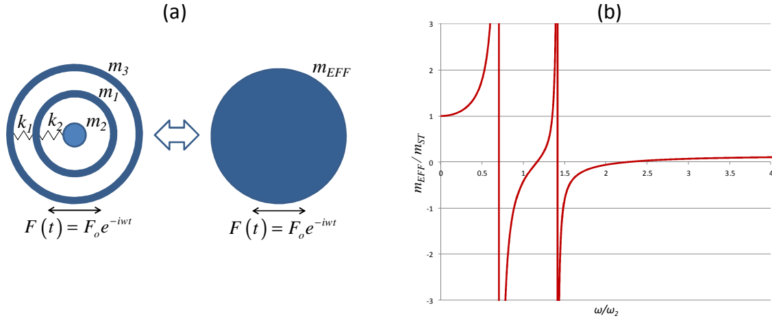
Fig. 1: (a) Dual-resonator spring-mass system and its effective mass model, (b) Plot of m_{EFF}/m_{ST} against \omega/\omega_2 .
