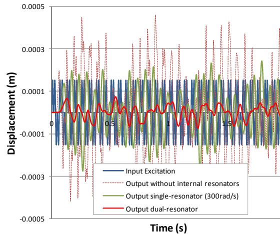
Fig. 2: Vibration control output responses using different microstructures.
