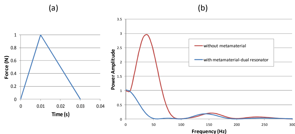
Fig. 3: (a) Input blast pulse, (b) Frequency domain by Fast Fourier Transform.
